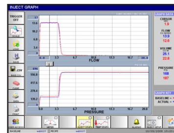
Wax Flow
