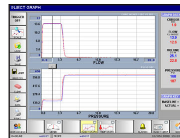
Wax Pressure
